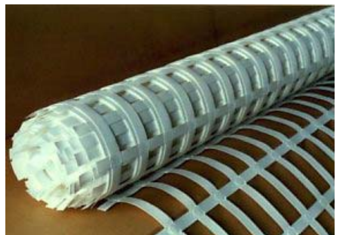
PARARIB is shipped in rolls of various widths and is relatively easy to transport and store on site.
